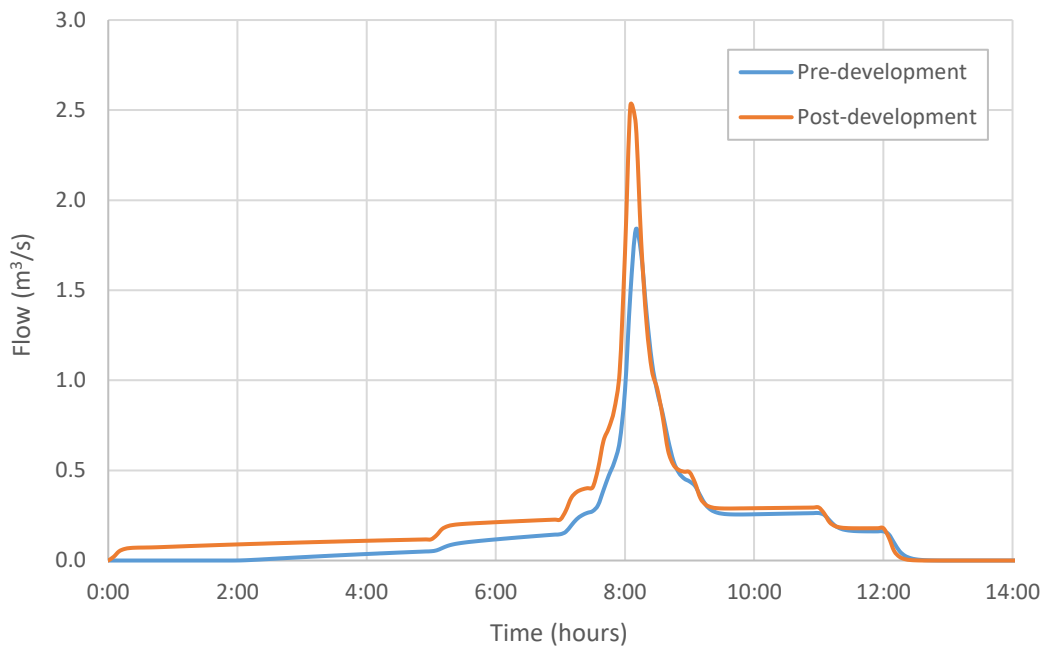
Figure 4-7 Pre- and post-development flood hydrographs in 1% AEP (including an allowance for climate change) nested storm flood event
